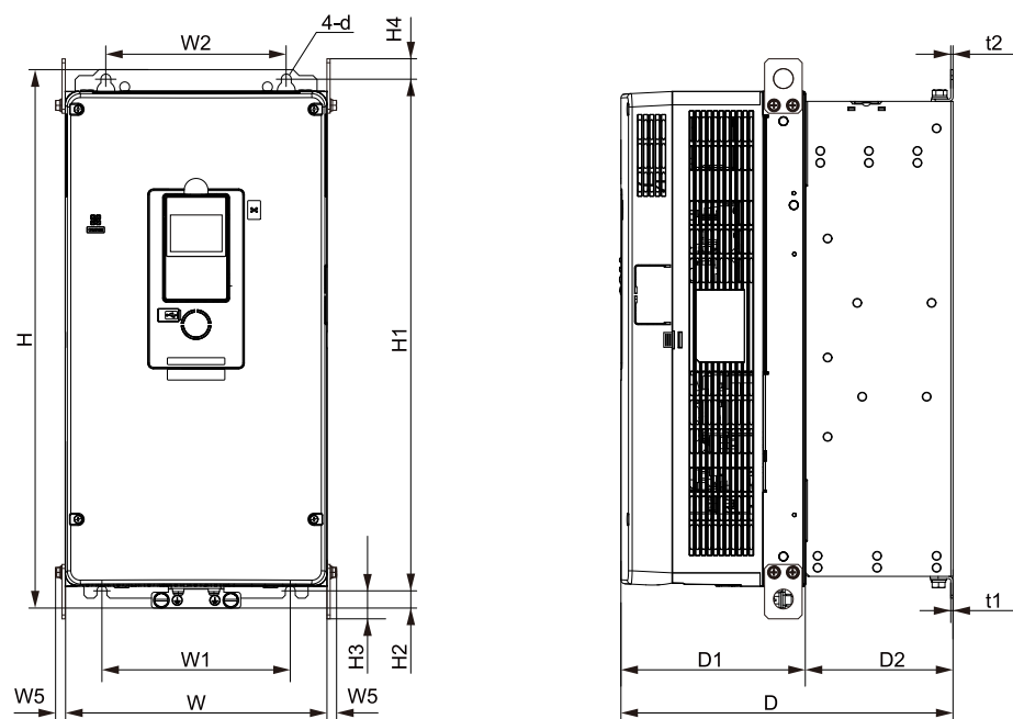
Figure 8.6 Dimension Diagram 6
